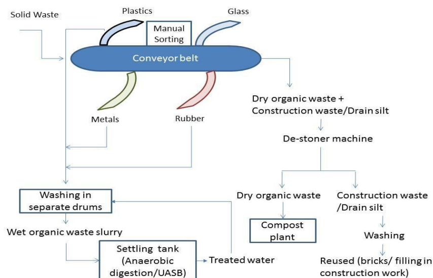
figure 4.01: Layout Showing Unit Operations of Sorting Station
